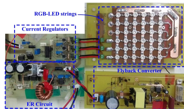
紅藍綠光-LED驅動器 Red, Blue, Green-LED driver
